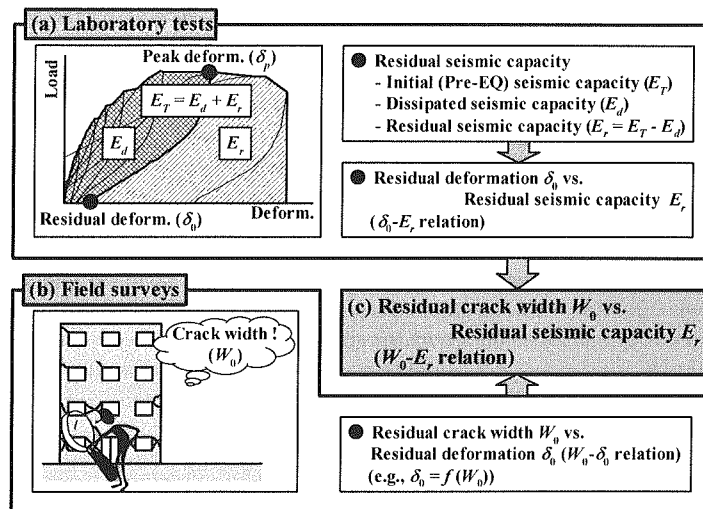
Figure 3: Basic concept of residual seismic capacity evaluation
