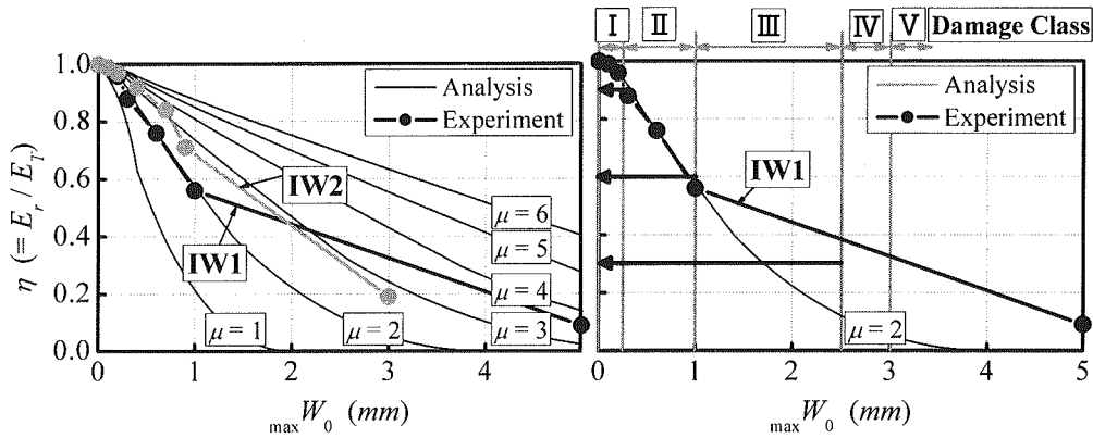
Figure 10: Relationship of \eta and \max W_0 of CB wall
