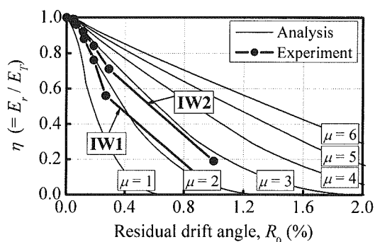
Figure 9: Relationship of R_0 and \eta
