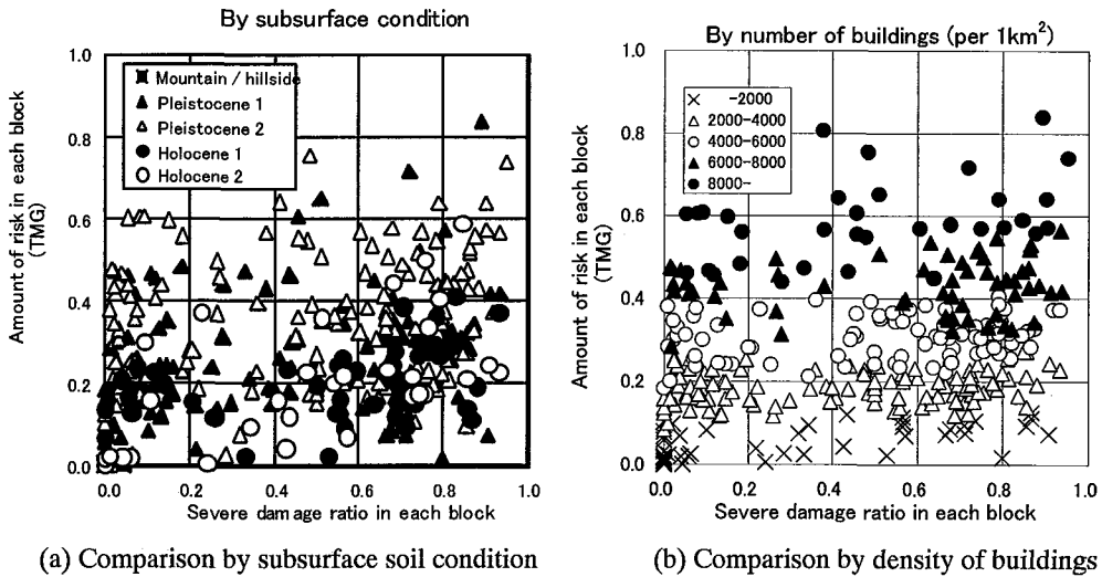
Fig. 3 Comparison between the collapse risk (TMG) and the actual damage due to the Kobe Earthquake in Nada Ward
