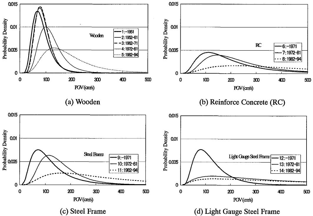
Fig. 4 Probability density functions for the seismic resistance of buildings with respect to PGV
