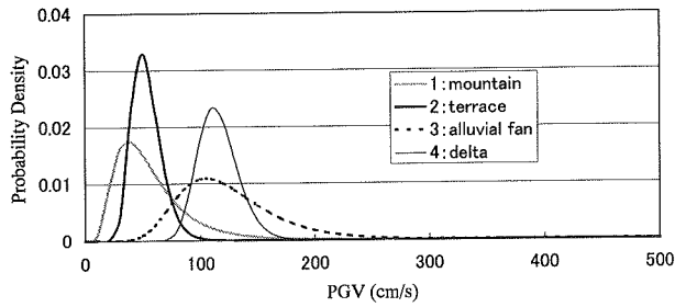
Fig. 5 Probability density function of the estimated PGV in the 1995 Kobe Earthquake for different topographical conditions in Nada Ward
