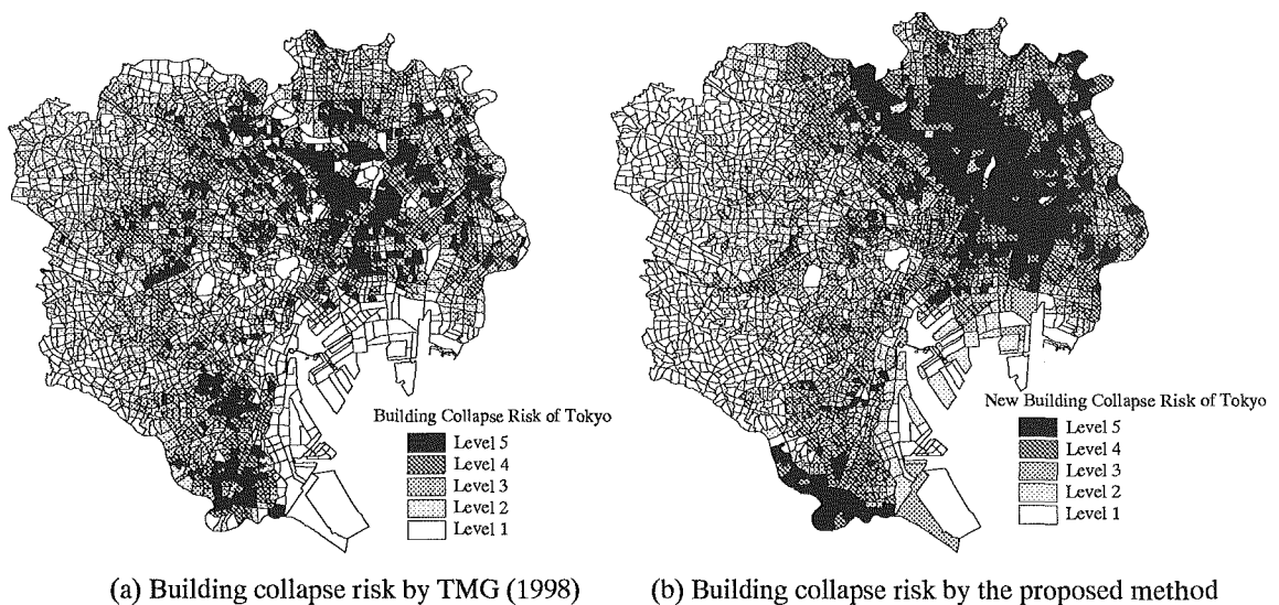
Fig. 7 Comparison of building collapse risk in Tokyo by two methods
