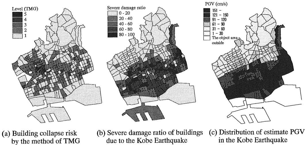
Fig. 2 Building collapse risk and actual damage in Nada Ward
